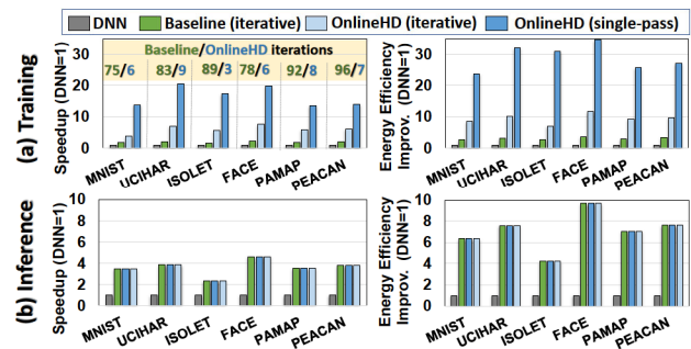
Figure 8: OnlineHD efficiency vs. state-of-the-art.
