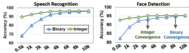
Figure 4: OnlineHD accuracy using binary or integer models.
