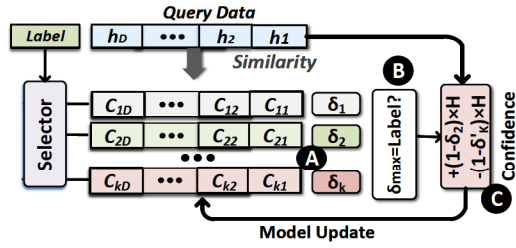
Figure 2: OnlineHD single-pass & adaptive iterative training.
