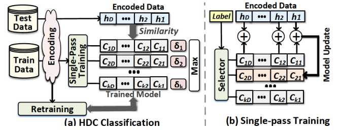
Figure 1: HDC classification steps & single-pass training.
