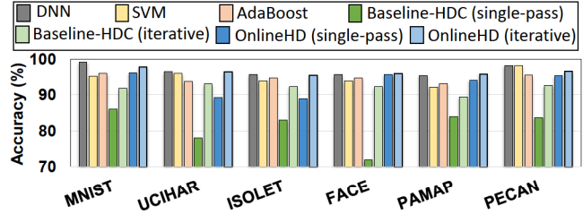
Figure 6: Comparing OnlineHD accuracy to state-of-the-art.
