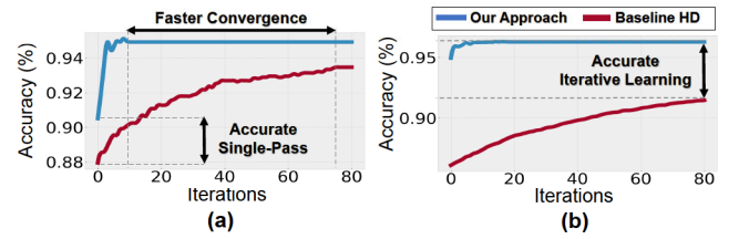
Figure 3: OnlineHD and baseline accuracy during retraining iterations: (a) speech recognition, (b) activity recognition.
