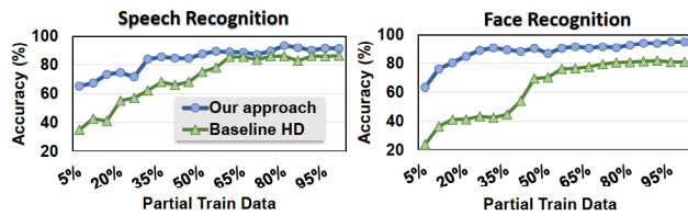
Figure 7: OnlineHD partial single-pass training.
